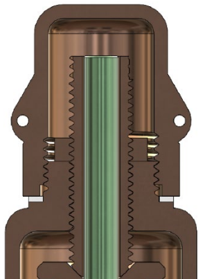
(A) Closed screwed cap
