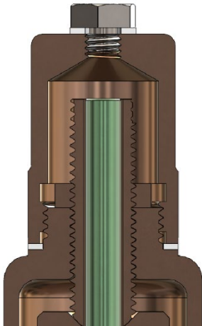
(B) Closed screwed cap + test gag
